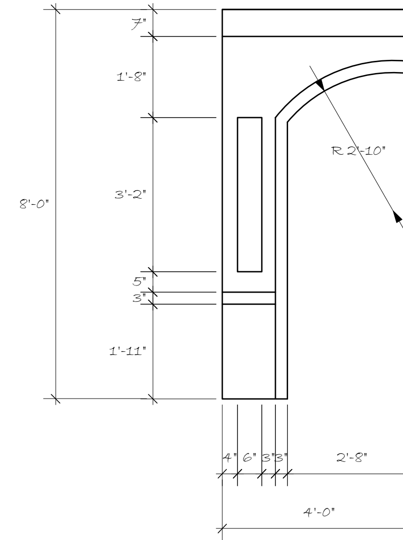
TRAIN SIDEWALL
